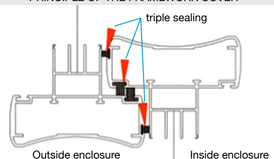
PRINCIPLE OF THE FRAMEWORK COVER
