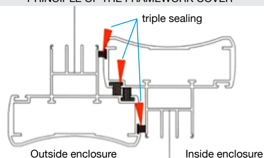
PRINCIPLE OF THE FRAMEWORK COVER
